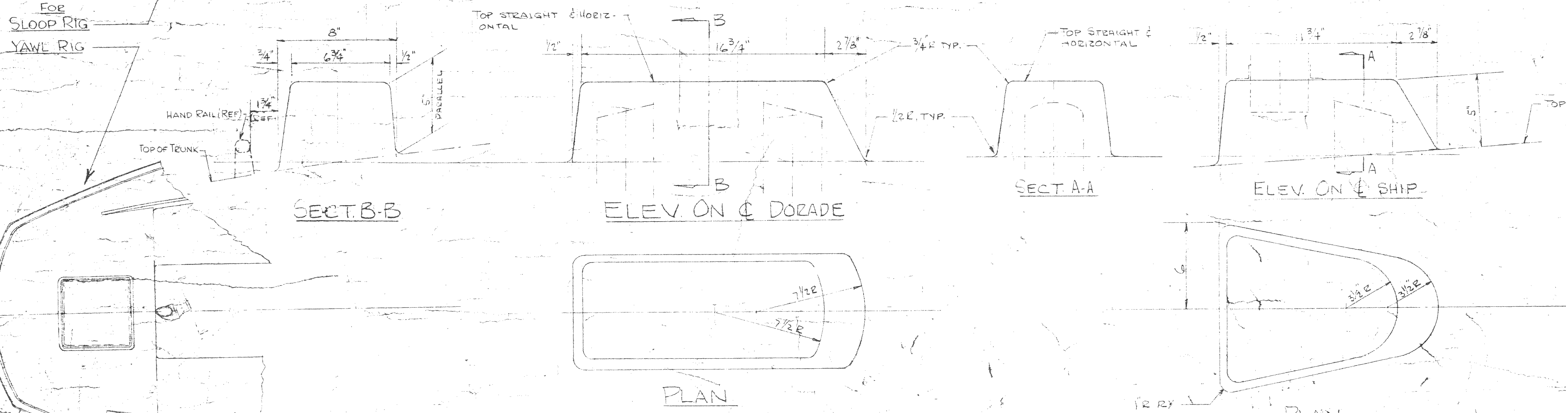
STB. TRUNK CABIN DORADE SCALE: 3/8" = 1'-0" 2 REQ'D. 1 EA. PORT & STB. PORT SIDE SIM. OFF. H&D FORE DECK DORADE SCALE: 3/8" = 1'-0"
